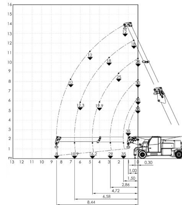
FRONT OUTRIGGERS
