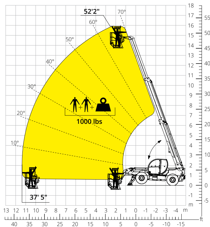
Load chart with PLATFORM, 1,000 lb, FOR MINES AT-01-027
